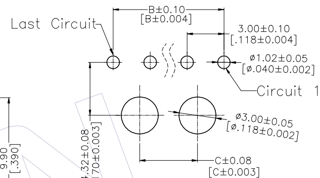
4-12 Circuit PCB LAYOUT
