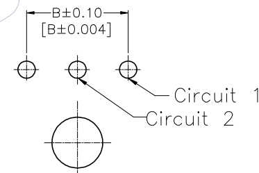
2-3 Circuit PCB LAYOUT
