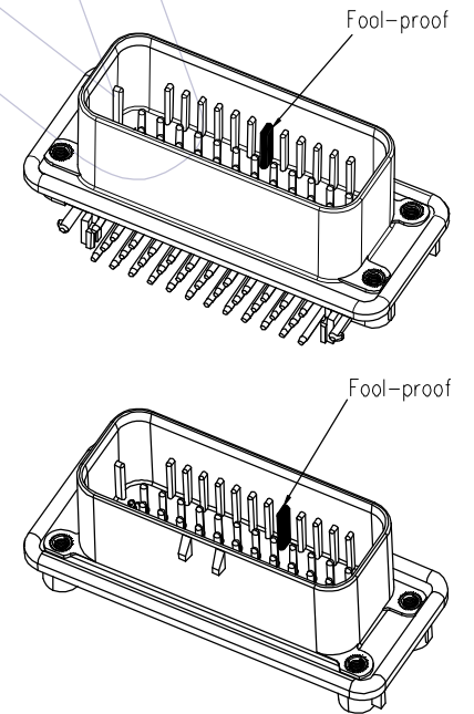
Fool-proof Structure
